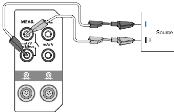
Figure 9 Current measurement
